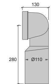
C + K3 WC - Stos, Universal, 110 muff RSK 310 66 87
